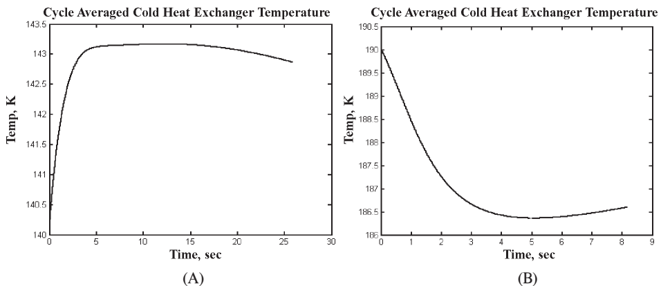
Figure 6. Cycle-averaged cold heat exchanger temperatures, mesoscale models; (A) ITPTR and (B) Reservoir-less ITPTR.
