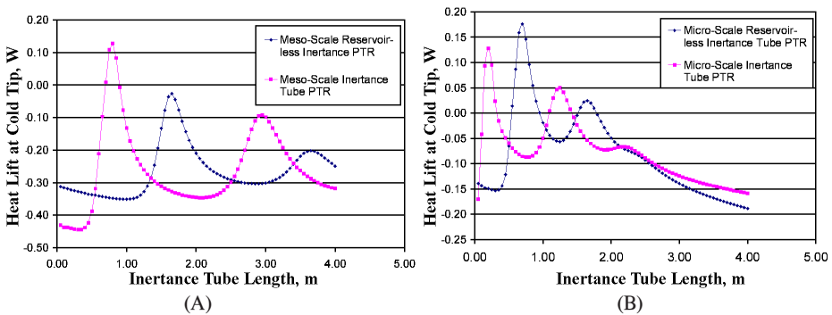
Figure 4. (A) Micro-scale and (B) Mesoscale PTR performance versus inertance tube length.
