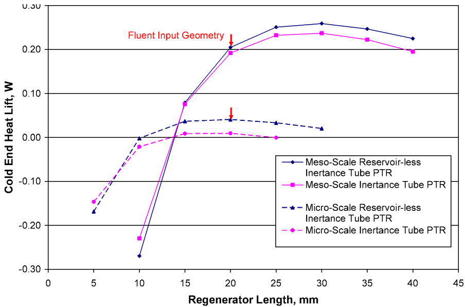
Figure 3. Map of PTR performance versus regenerator length.
