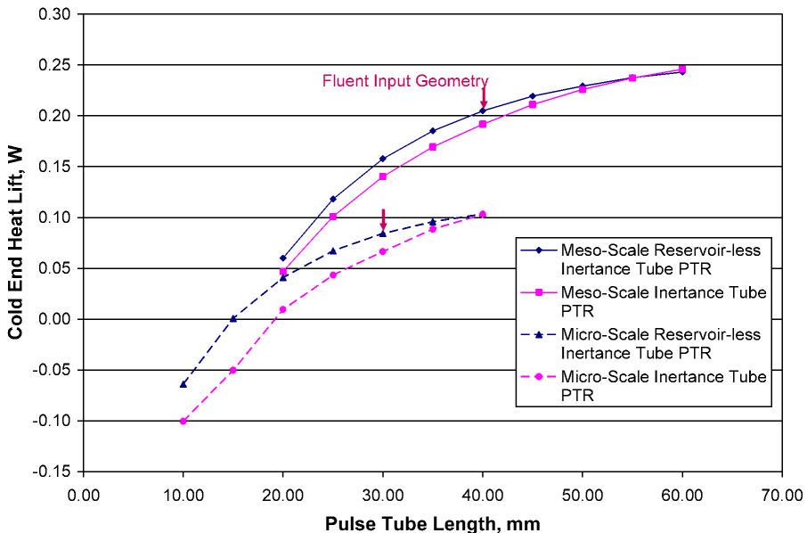
Figure 2. Map of PTR performance versus pulse tube length.
