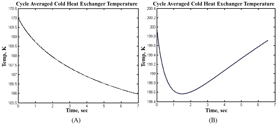
Figure 7. Cycle-averaged cold heat exchanger temperature histories, micro-scale models; (A) ITPTR and (B) Reservoir-less ITPTR.
