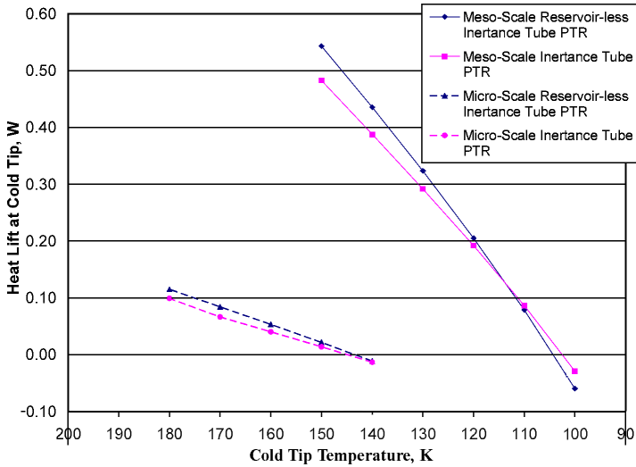
Figure 5. Load curves for micro-scale and mesoscale Sage PTR models.
