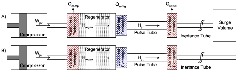
Figure 1. Schematics of modeled PTRs; (A) Inertance Tube PTR, (B) Reservoirless Inertance Tube PTR.
