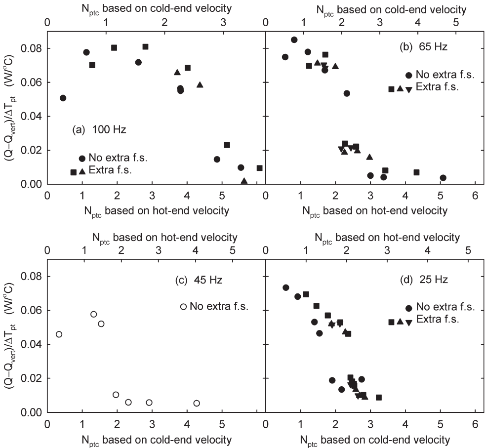
Figure 6. Convection conductance vs pulse-tube convection number, at four different frequencies, in the tube of Fig. 2(d) with 3.1-MPa helium gas and T_{hot} = 250^\circ\text{C} . The primary horizontal axes, which all run from 0 to 6.25, use the fastest velocity in the tube, and the upper horizontal axes use the slowest velocity. Unfilled symbols are used for the lone case of steady convection in this figure, and filled symbols denote time-dependent convection.
