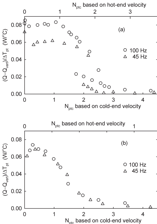
Figure 5. Convection conductance vs pulse-tube-convection number at two frequencies in 3.1-MPa helium. On the bottom axes, N_{ptc} is calculated using the velocity at the cold end of the pulse tube, where the velocity is highest. Auxiliary (top) axes show how different that axis would be if the hot end were used. (a) Measurements with the setup of Fig. 2(c), i.e., a relatively low p_a/p_m and low end-to-end velocity variation. The 100-Hz data are also shown in Fig. 3. (b) Measurements with the setup of Fig. 2(a), i.e., with a higher p_a/p_m and higher end-to-end velocity variation. (These data also appear in Ref. 4, Fig. 4(b), where the mid-tube velocity was used.)
