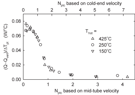
Figure 4. Convection conductance vs N_{ptc} for three different hot temperatures, all with T_{cold} \sim 20^\circ\text{C} , in 3.1-MPa helium at 100 Hz in the setup of Fig. 2(a). These are the same data shown in Ref. 4, Fig. 5(b), but here using \Delta T_{pt} instead of the thermocouple temperature difference in the horizontal axis. This graph uses \beta = 1/2 in N_{ptc} . As shown in Ref. 4, using \beta = 1 ruins the agreement among the three data sets.
