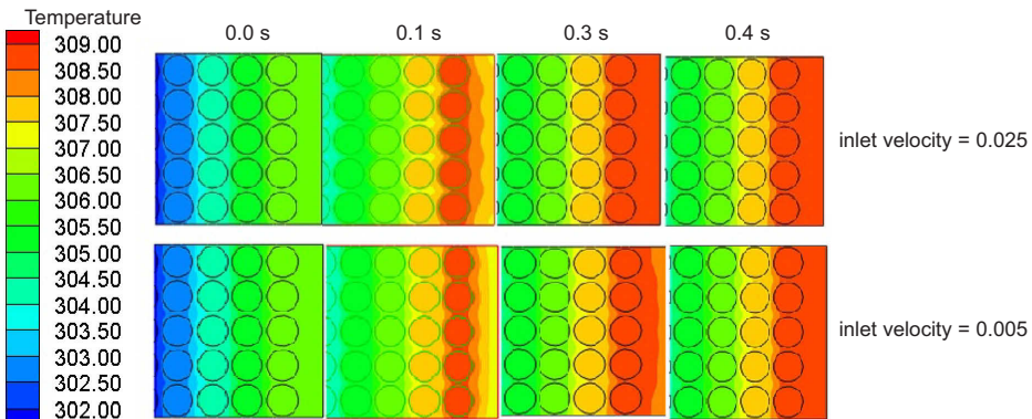
Figure 2. Temperature field for the heat transfer course under different inlet velocities.
