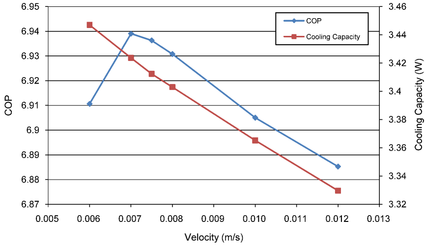
Figure 6: Velocity vs. COP and cooling capacity for \Delta T_{\text{span}} = 40\text{K} .
