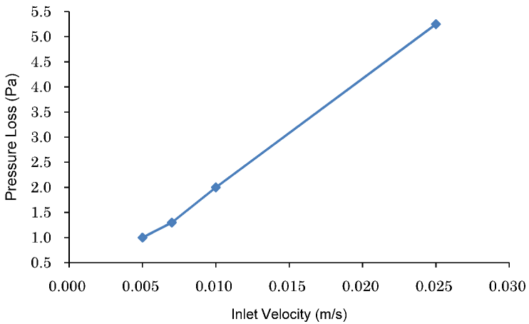
Figure 5. Pressure loss vs Inlet velocity for \Delta T_{span} = 40 K
