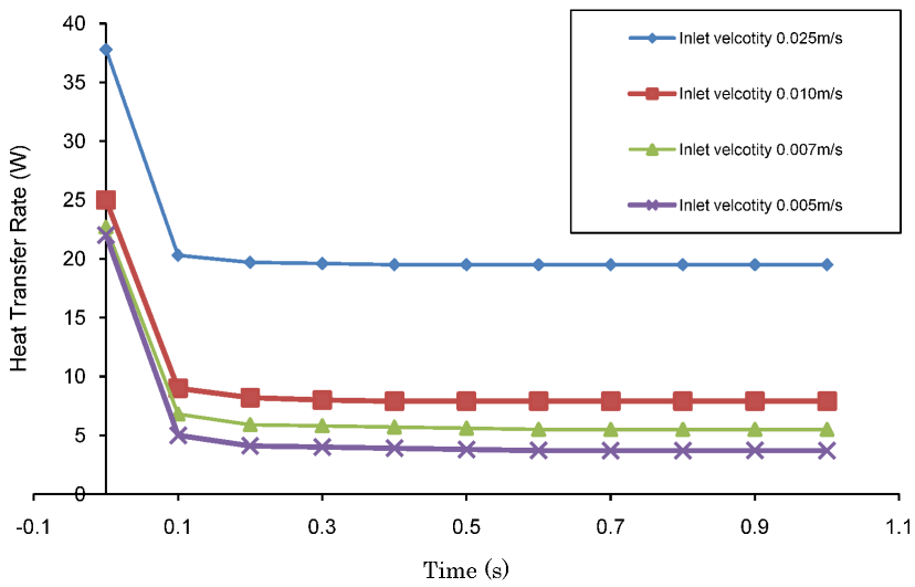
Figure 4. Heat transfer rate Vs. Time for different velocities ( \Delta T_{span} = 40 K)
